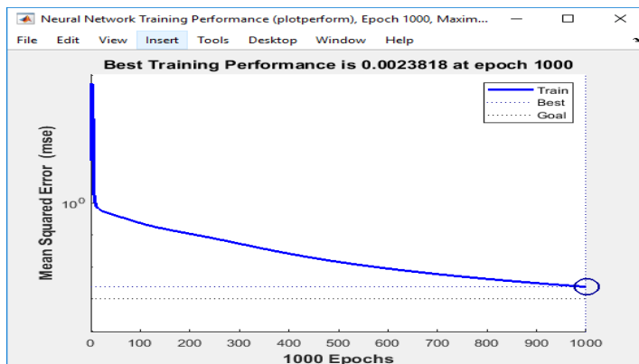
Figure3.2. Dependence graph of the training error- "mse"for the real object as a "black box" on the number of "epochs" (a) and description of NN in Simulink as a subsytem (b)
